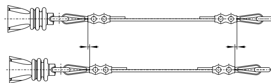
Image 4: deformation of the wire thimbles
